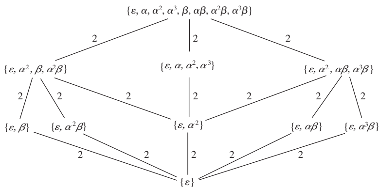
Figure 32.1 Lattice of subgroups of the group of field automorphisms of Q(\sqrt[4]{2}, i) , where \alpha: i \rightarrow i and \sqrt[4]{2} \rightarrow -i\sqrt[4]{2} , \beta: i \rightarrow -i , and \sqrt[4]{2} \rightarrow \sqrt[4]{2} .
