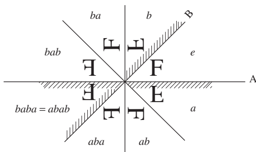
Figure 26.2 The group D_4 —reflections in mirrors at a 45^\circ angle
