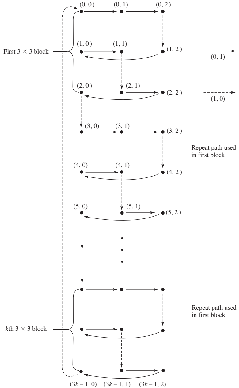
Figure 30.6 Cay(\{(1, 0), (0, 1)\}; Z_{3k} \oplus Z_3) .
