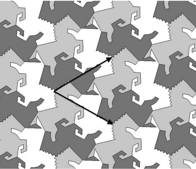
Figure 28.14 Horses 1 by Makoto Nakamura, adapted by Kevin Lee. Design with symmetry group p3 (disregarding shading). The inserted arrows are translation vectors.
