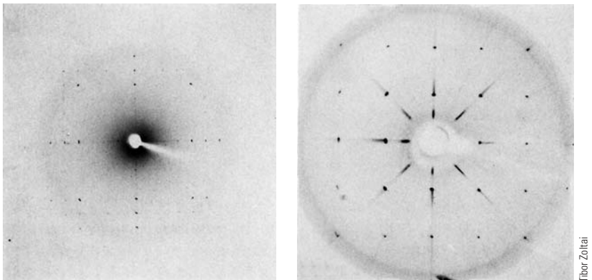
Figure 1.3 X-ray diffraction photos revealing D_4 symmetry patterns in crystals.
